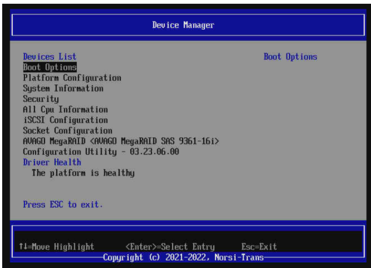
Рис. 67. Меню Device Manager
