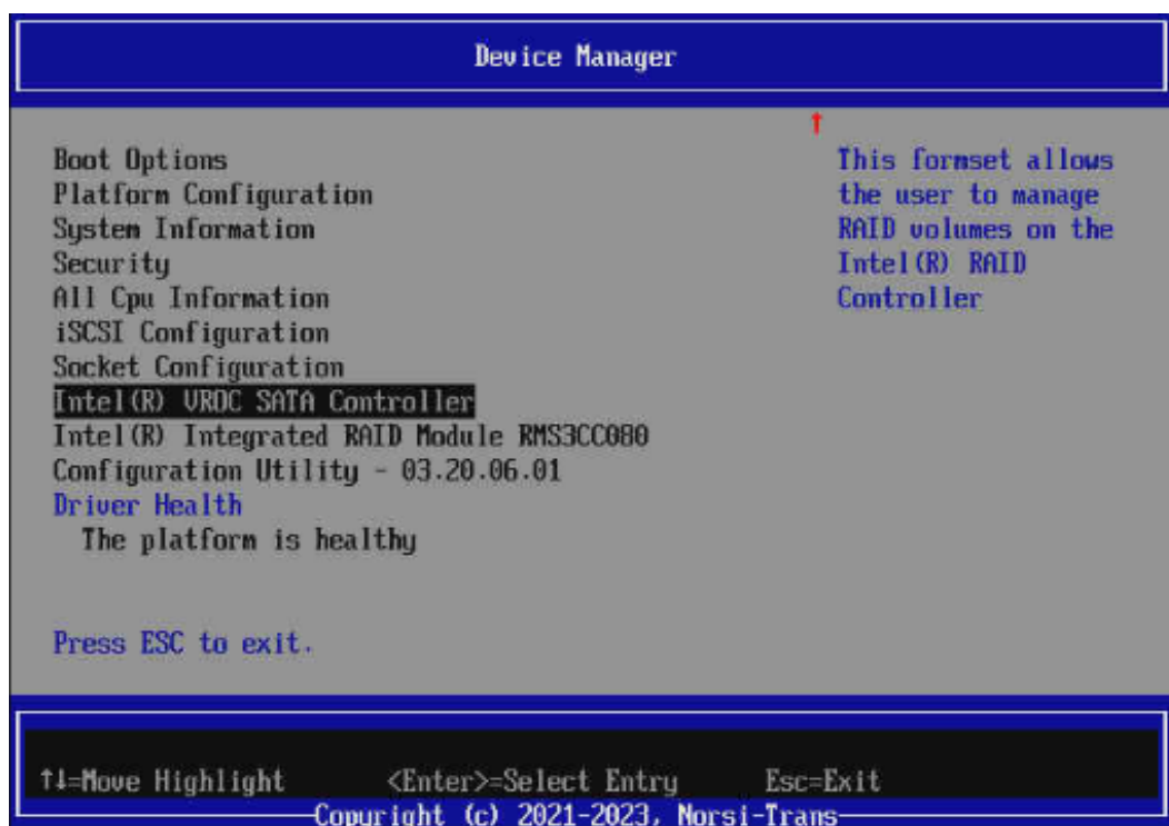
Рис. 73. Меню Device Manager
